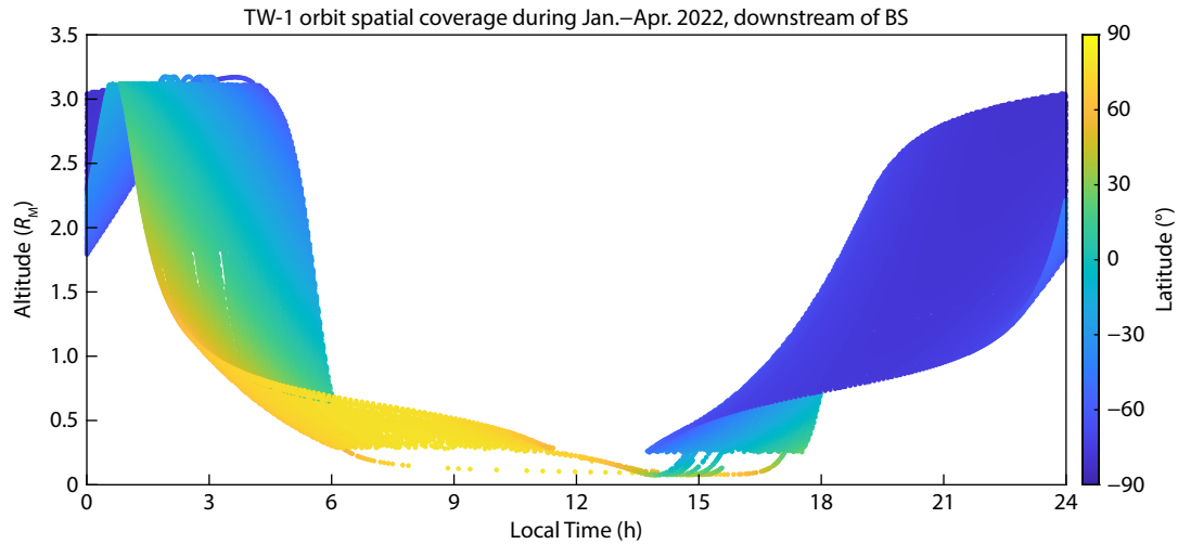
Figure 3. Spatial coverage of the investigated dataset. TW-1, Tianwen-1; BS, bow shock.
