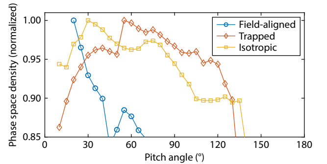
Figure 2. Example of the three types of distribution. The blue line with circles shows a field-aligned distribution, sampled on January 16, 2022, at 22:28, A = -1.98 ; the red line with diamonds shows a trapped-like distribution, sampled on January 23, 2022, at 05:10, A = 2.83 ; and the orange line with squares shows an isotropic distribution, sampled on January 23, 2022, at 05:11, A = 0.18 .
