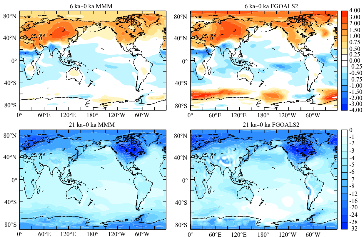
Figure 12. The surface air temperature (SAT) simulation by FGOALS for the paleoclimate simulation of the mid-Holocene (6 ka, above) and Last Interglacial Maximum (21 ka, below). MMM denotes the multi-model mean. Unit: °C (after Zheng WP et al. 2013b).
