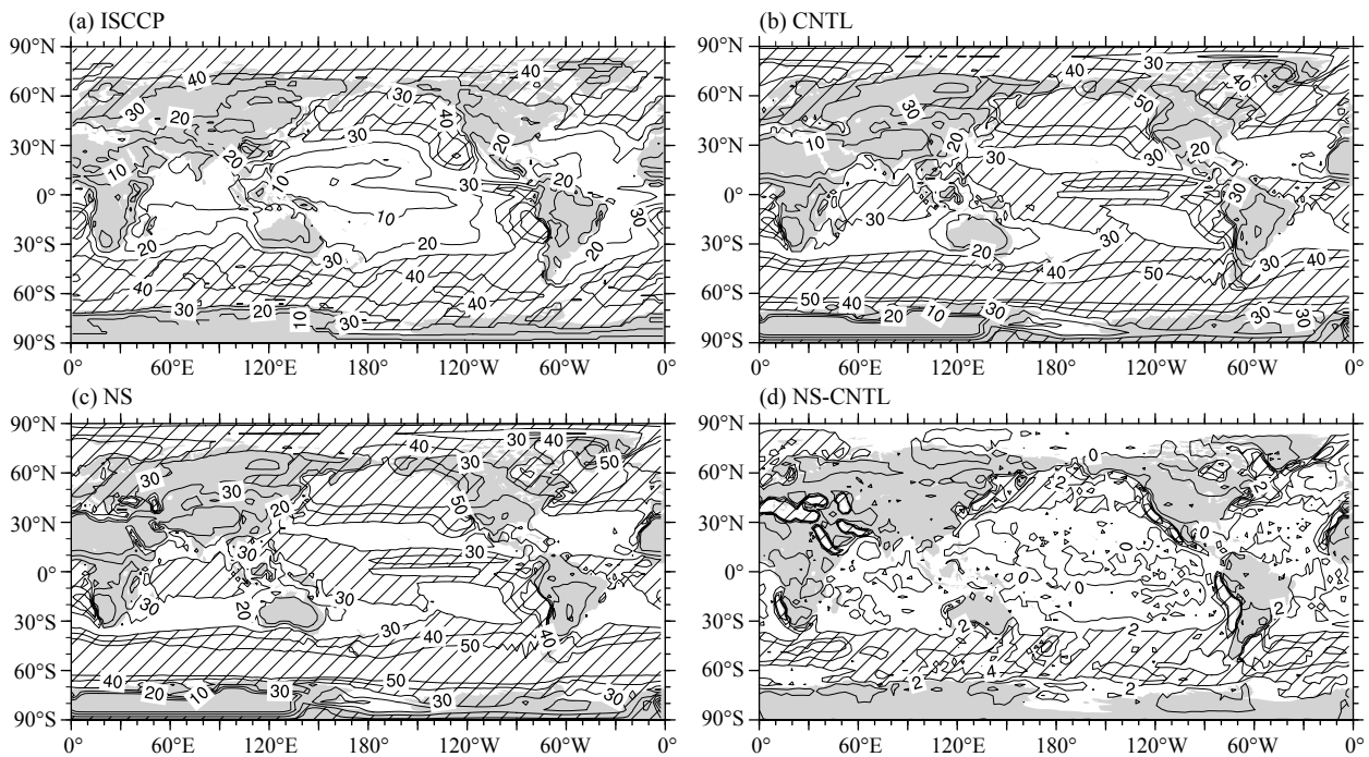
Figure 3. Annual mean low-level stratiform cloud fraction (%). (a) ISCCP; (b) GAMIL2 with original stratocumulus scheme; (c) GAMIL2 with a modified stratocumulus scheme; (d) Differences in cloud amount between (b) and (c).
