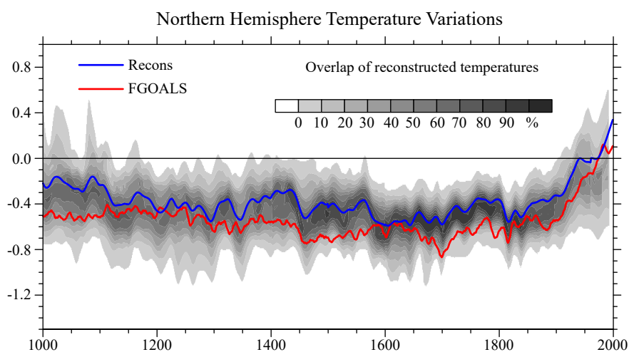
Figure 13. Low-pass filtered North Hemispheric (NH) mean surface temperature changes (°C) during the past millennium. The mean of the reconstructions is shown as the blue line, and the simulated time series is shown as the red line. The gray shading indicates the overlap of the uncertainty ranges of the NH reconstructions, as in Figure 6.13d of IPCC AR4 (Jansen et al., 2007). The anomalies are calculated with respect to the climate mean of the 1961–1990 reference period. Fluctuations at time scales less than 30 years have been removed (redrawn based on Man WM and Zhou TJ, 2014a).
