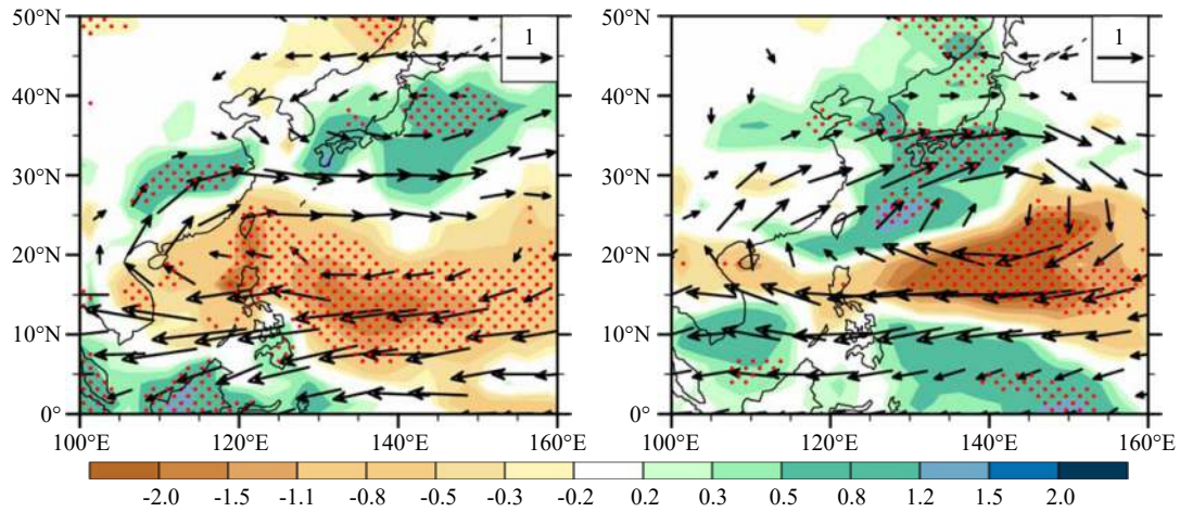
Figure 7. East Asian summer monsoon in El Niño decaying summer derived from reanalysis (left) and FGOALS-s2 simulation (right, redrawn based on Song FF and Zhou TJ, 2014a).
