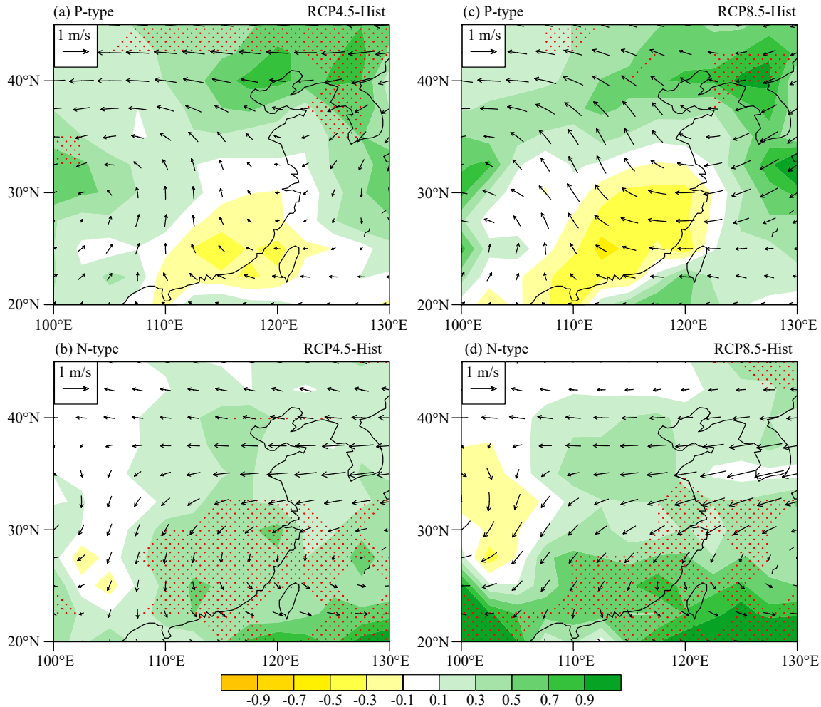
Figure 14. (a) P-type models' composite of the projected changes in precipitation (shading, unit: mm/day) and 850 hPa wind (vectors, unit: m/s) under the RCP4.5 scenario. (b) Same as (a) but for the N-type models. (c–d) Same as (a–b) but under the RCP8.5 scenario. The models that project significantly enhanced (decreased) western North Pacific subtropical high intensity are referred as P-type (N-type). The red dots indicate regions for which all of the P-type (or N-type) models agree in the sign of changes in precipitation (after He C and Zhou TJ, 2015).
