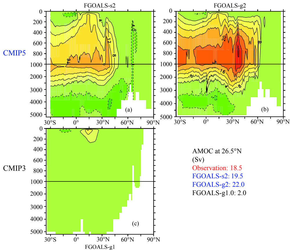
Figure 9. AMOC (Sv, 1 Sv=10 6 m 3 /s) simulated by FGAOLS versions for CMIP3 and CMIP5. The AMOCs at 26.5°N for CMIP5, CMIP3 versions and RAPID data are shown (after Lin PF et al., 2013a).
