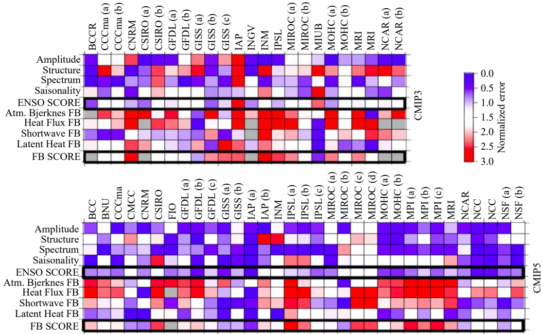
Figure 5. ENSO skills in CMIP3 and CMIP5 models (Figure 13 from Bellenger et al. (2014)).
