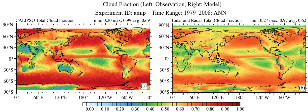
Figure 2. Geographical distribution of total cloud fraction for (a) CALIPSO observations and (b) GAMIL2 using the CALIPSO satellite simulator (from Li LJ et al., 2014a).
