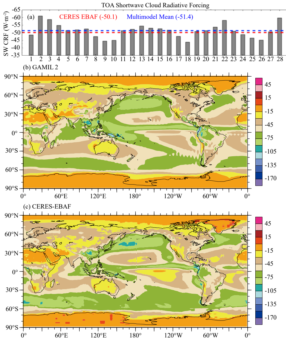
Figure 4. (a) Near global (65°S–65°N) mean shortwave cloud radiations forcing at the top of the atmosphere from 28 CMIP5 models, multimodel mean (blue) and satellite observation (red) CERES EBAF, and the geographical distribution for GAMIL2 (b) and CERES EBAF (c). Model number 11 is GAMIL2. (Figure (a) from Dolinar et al., 2015; Figures (b) and (c) redrawn based on Li LJ et al., 2013a).
