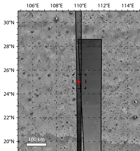
Figure 1. Mosaic map of OMEGA (Observatoire pour la Minéralogie, l'Eau, les Glaces et l'Activité) albedo data at 2.32\text{ }\mu\text{m} covering the landing site (red cross symbol) and surrounding area. The swaths on the left and right are orb0973_5 and orb2257_4, respectively, superimposed on the THEMIS (Thermal Emission Imaging System) map. The black dashed box indicates the area shown in Figures 2 and 4.
