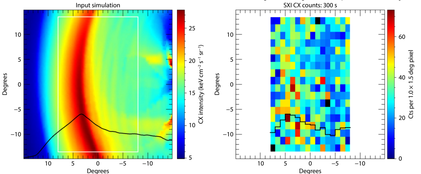
Figure 4. SXI image simulation, 0.2 to 1.1 keV, for a solar wind flux case of 4.9 \times 10^8 \text{ cm}^{-2} \text{ s}^{-1} .
