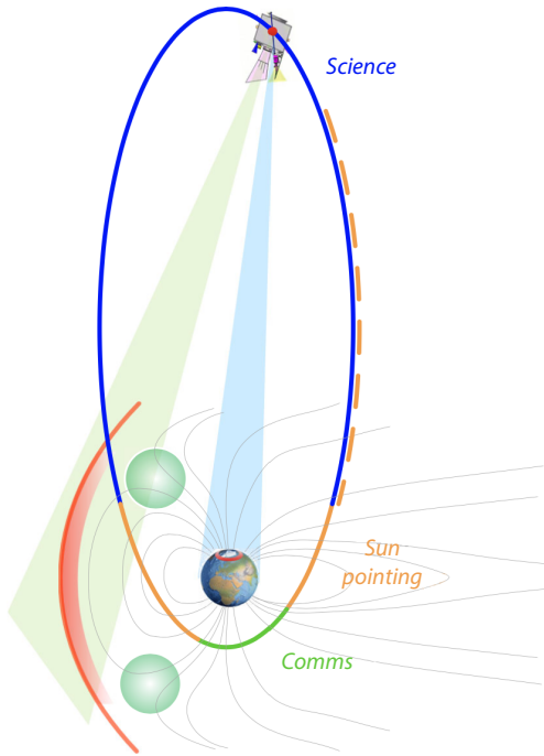
Figure 2. Schematic (not to scale) of the SMILE orbit (source ESA) with the three main orbital phases shown. SXI science phase is shown in blue. Main communications (download and upload) occurs during perigee passage (green). During the phases shown in orange SXI and UVI operations may not be allowed due to Sun exclusion constraints. This is time of year dependent as illustrated by the dashed orange line. The SXI science target is the magnetosheath (left of figure) and UVI science target is the footprint of the Northern magnetospheric cusp.
