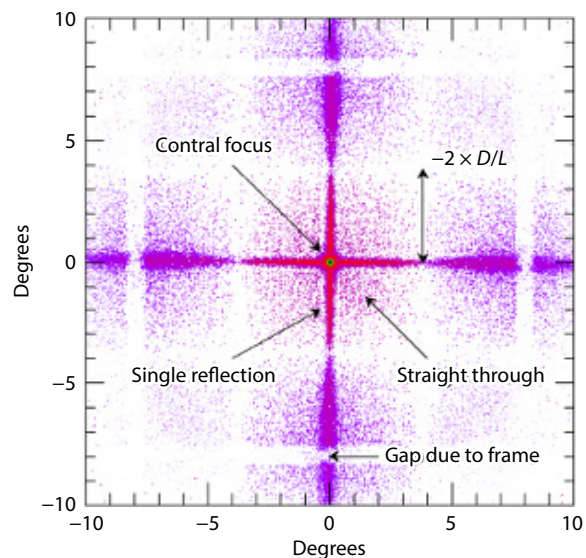
Figure 3. (Left) Diagram showing the basic principle of the Lobster-eye optic geometry. Parallel beams of X-rays are brought to a focus at half the radius of curvature ( R ) of the hemi spherical optic array. (Right) Simulation of the MPO PSF at 0.5 keV. The intensity of the image is on a logarithmic scale and the central focus is saturated. D/L is the ratio of the channel width (40 microns) to the channel length (1.2 mm) and defines the angular scale of the inner cross arms.
