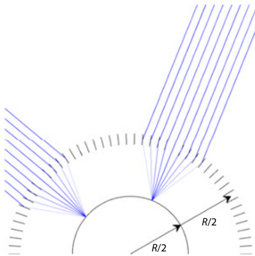
Figure 3. (Left) Diagram showing the basic principle of the Lobster-eye optic geometry. Parallel beams of X-rays are brought to a focus at half the radius of curvature ( R ) of the hemi spherical optic array. (Right) Simulation of the MPO PSF at 0.5 keV. The intensity of the image is on a logarithmic scale and the central focus is saturated. D/L is the ratio of the channel width (40 microns) to the channel length (1.2 mm) and defines the angular scale of the inner cross arms.
