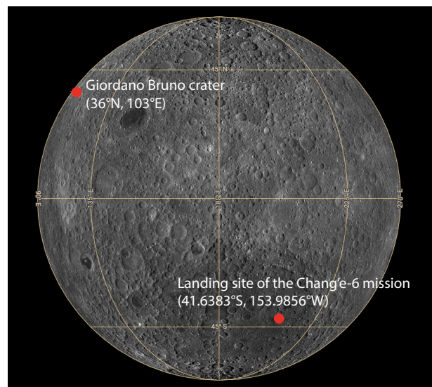
Figure 2. Location of the Giordano Bruno crater and the landing site of the Chang'e-6 mission. The two red circles show the locations of the Giordano Bruno crater (the possible origin of Kamo'oalewa) and the landing site of the Chang'e-6 mission (Liu ZQ et al., 2024) on the farside of the Moon. The map of the lunar farside is from LROC (Lunar Reconnaissance Orbiter Camera) QuickMap ( https://quickmap.lroc.asu.edu/projections?prjExtent=-1594681.2981205%2C-909717.6478905%2C1594681.2981205%2C766092.1105477&showGraticule=true&layers=NrBsFYBoAZIRnpEBmZcAsjYIHfFcAbAyAbwF8BdCOyioA&proj=7 ).
