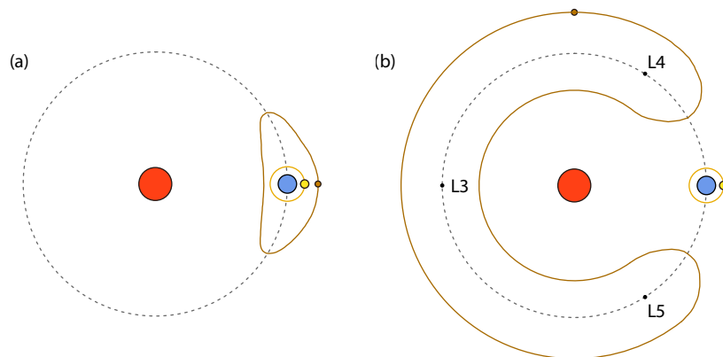
Figure 1. Two types of co-orbital states related to Kamo'oalewa (not to scale). (a) The co-orbital state (quasi-satellite) of Kamo'oalewa (brown line) at present. The red, blue, yellow, and brown circles represent the Sun, the Earth, the Moon, and Kamo'oalewa, respectively. The gray dashed line and the yellow line show the orbits of the Earth and the Moon, respectively. The distance of Kamo'oalewa from the Earth is 38 to 100 lunar distances, far from the sphere of gravitational influence of the Earth. (b) Kamo'oalewa will switch into a horseshoe orbit about 300 years later. L3, L4, and L5 are the three Lagrange points of the Sun–Earth system. Modified from Castro-Cisneros et al. (2023).
