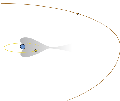
Figure 3. The current orbit of the Moon and Kamo'oalewa in the background of the Earth wind (not to scale). The blue, yellow, and brown circles represent the Earth, the Moon, and Kamo'oalewa, respectively. The yellow and brown lines show the orbits of the Moon and Kamo'oalewa. The main region of particles escaping from the Earth is shown in gray (Wei Y et al., 2020). Kamo'oalewa is 38 to 100 lunar distances away from the Earth, resulting in less influence than the Moon from particles escaping from the Earth.
